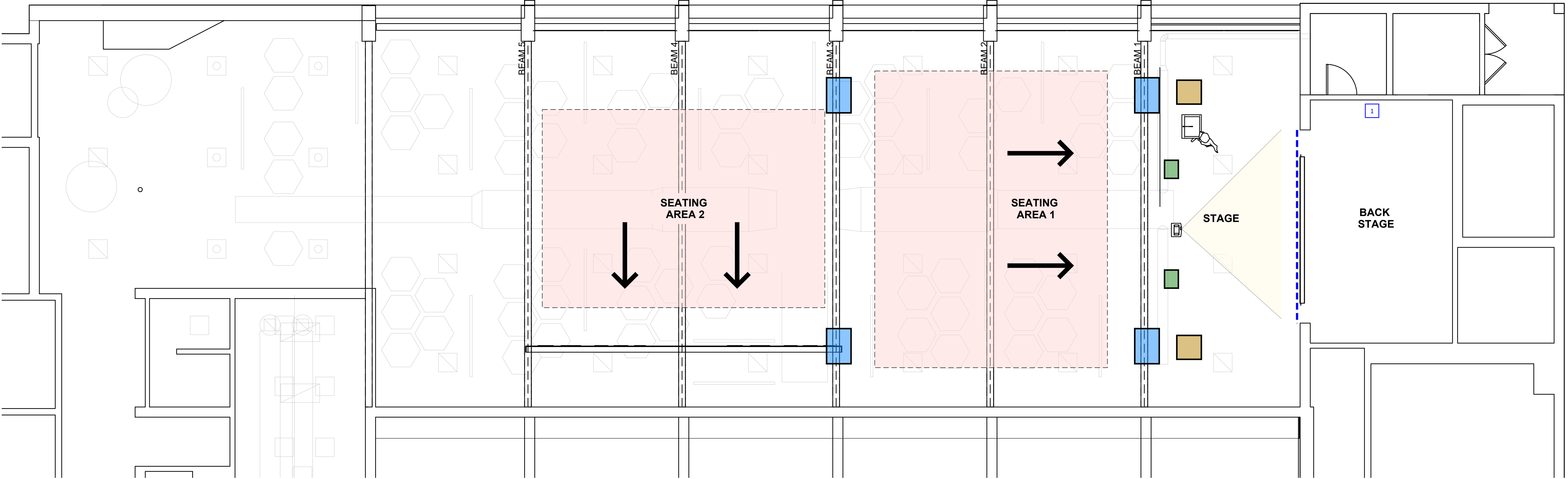
1 :: ENLARGED AUDITORIUM PLAN 1 scale: 3/16" = 1'-0"
